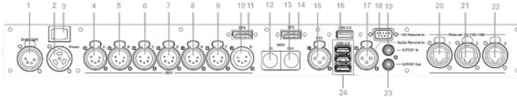
grandMA3 full-size back panel
